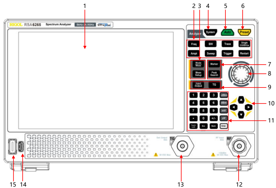
Figure 4.4 Front Panel
