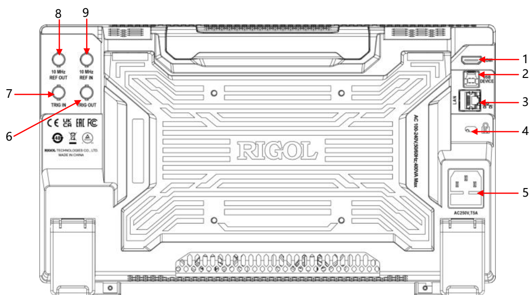
Figure 4.8 Rear Panel
