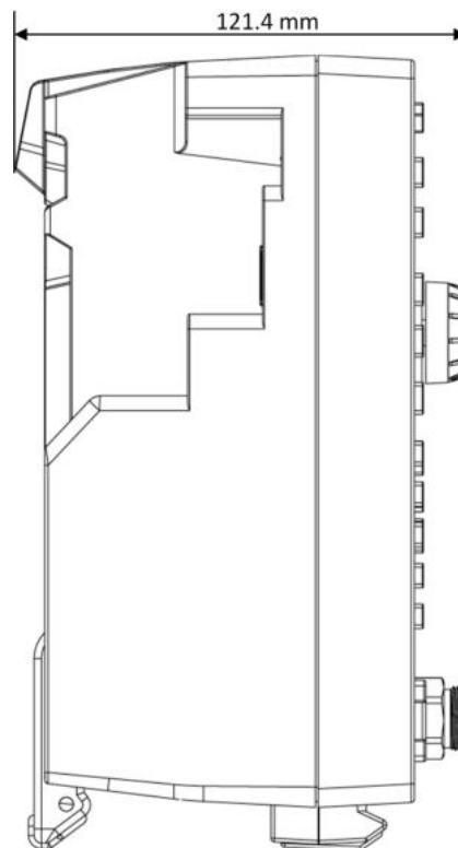
Figure 4.2 Side view (mm)
