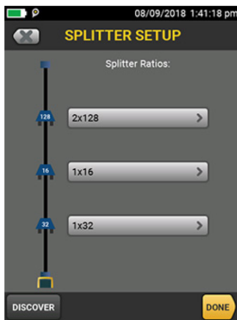
Splitter setup
