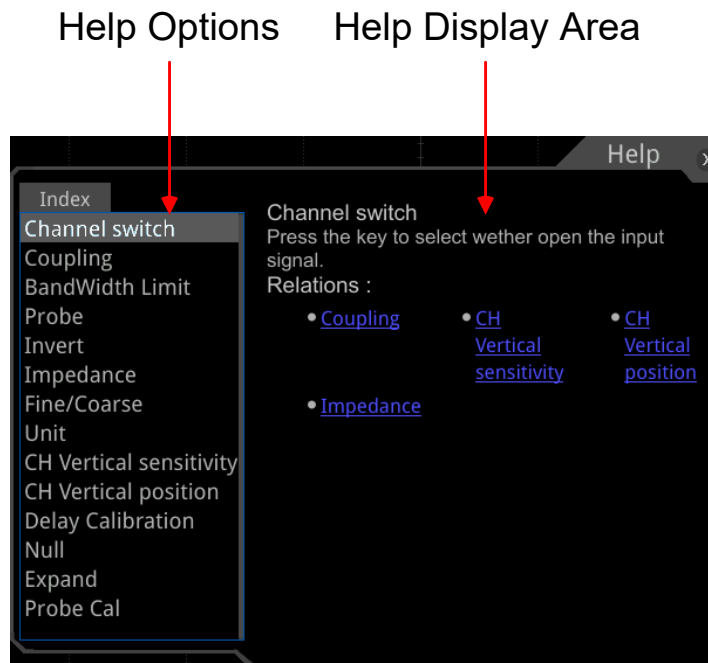
Figure 9.1 Help Information
