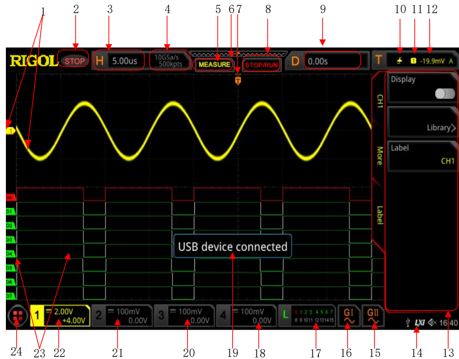
Figure 6.3 User Interface
