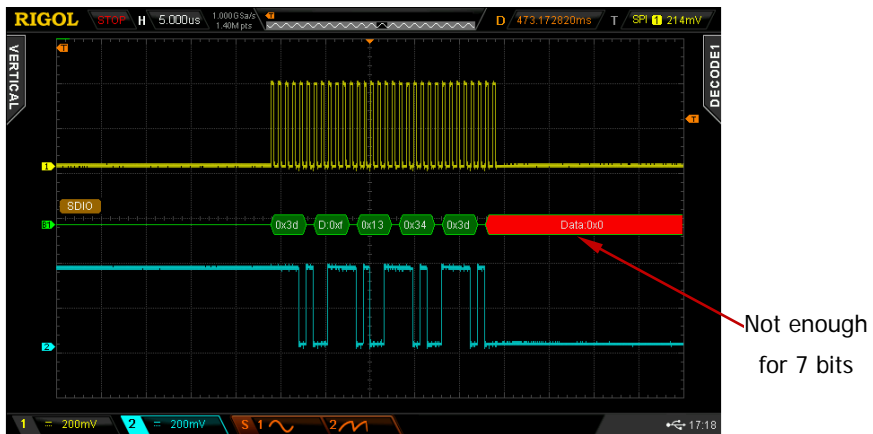
Figure 7-13 Error Expressions During Decoding
