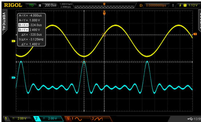
Figure 6-9 Cursor Track (Before Horizontal Expansion)
