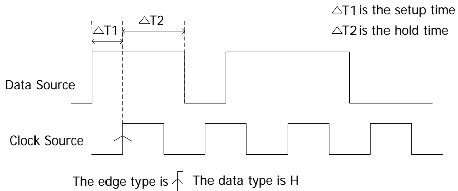
Figure 5-9 Setup/Hold Trigger
