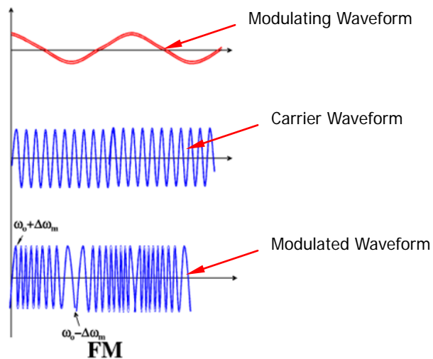
Figure 12-10 FM
