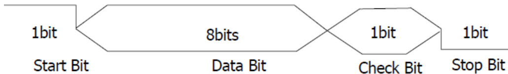
Figure 5-10 RS232 Trigger
