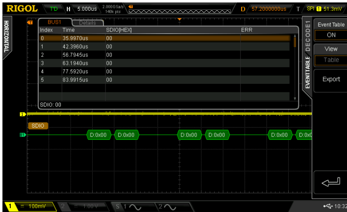
Figure 7-12 SPI Decoding Table
