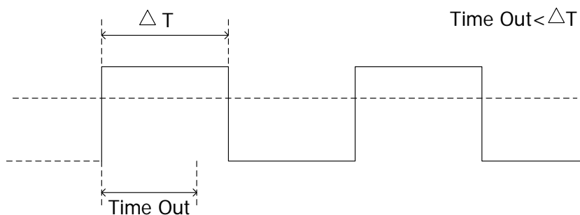
Figure 5-7 TimeOut Trigger
