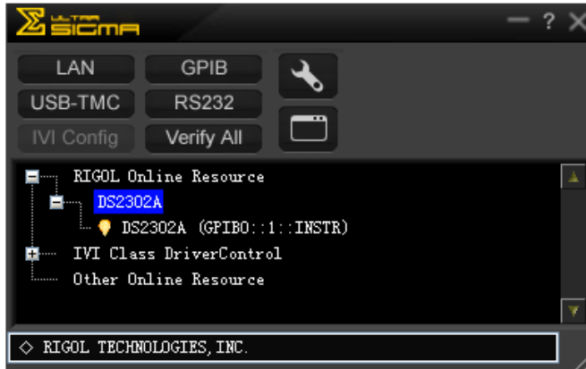
Figure 15-7 View the Device Resource under Control via GPIB
