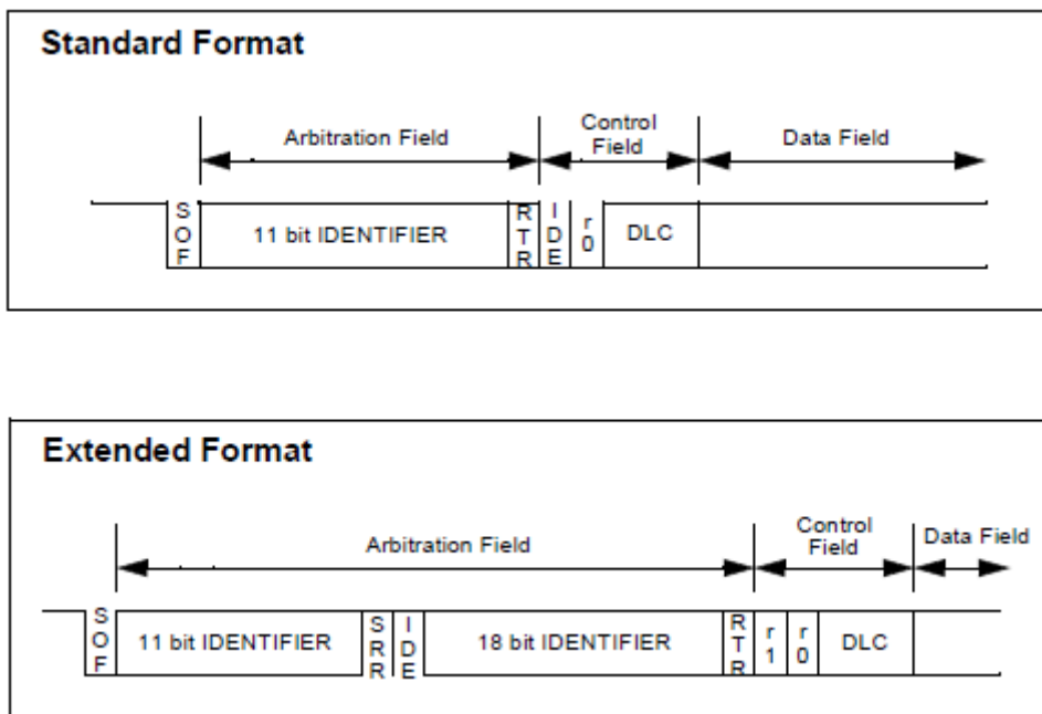
Figure 5-14 Standard and Expanded Formats of CAN Bus Data Frame
