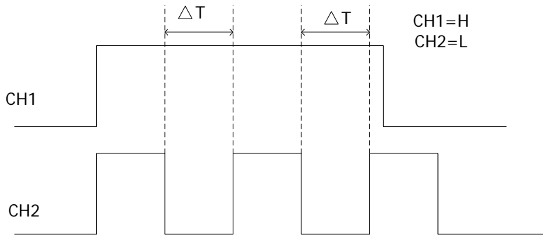
Figure 5-8 Duration Trigger
