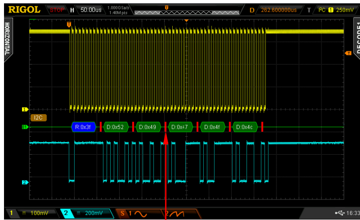
Figure 7-10 Error Expressions during Decoding
