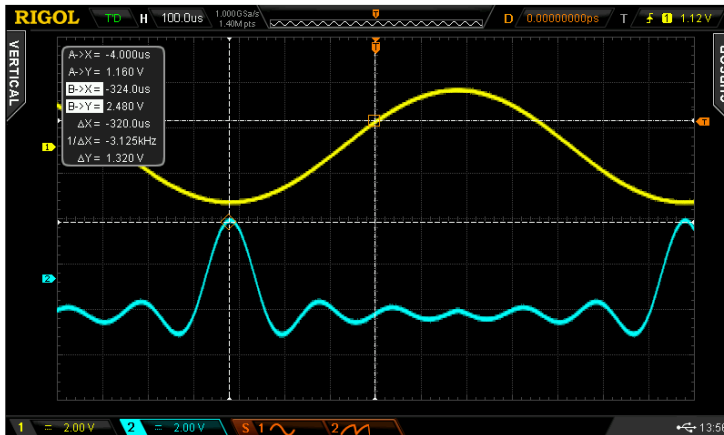
Figure 6-10 Cursor Track (After Horizontal Expansion)
