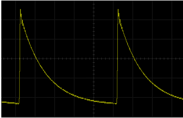
Figure 12-4 ExpFall Function Waveform
