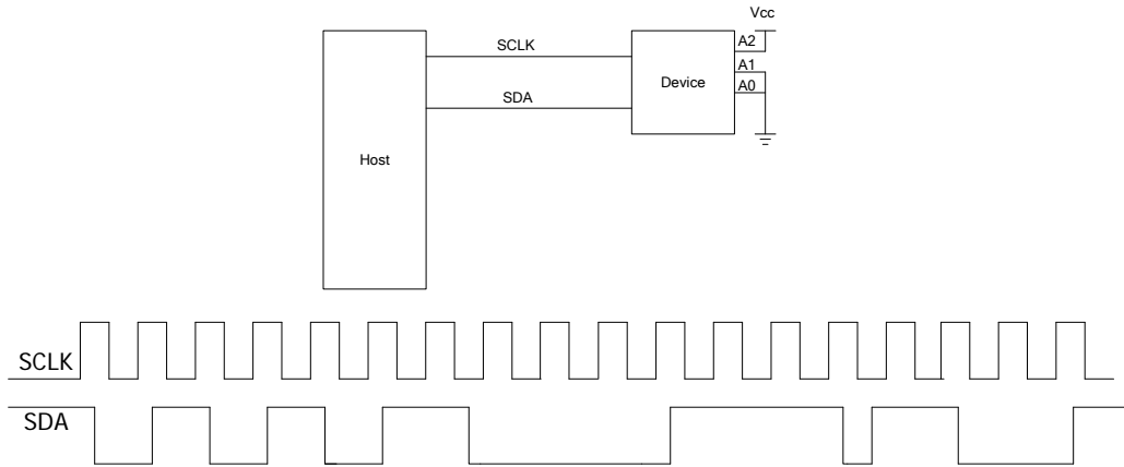
Figure 7-6 I2C Serial Bus
