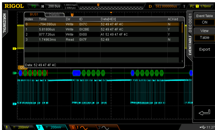
Figure 7-7 I2C Decoding Table (Table)
