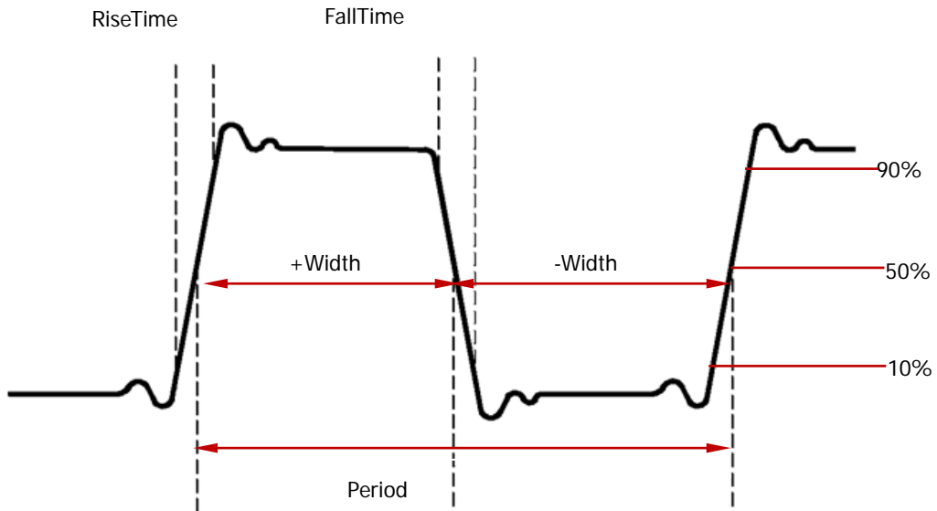
Figure 6-3 Time Parameters
