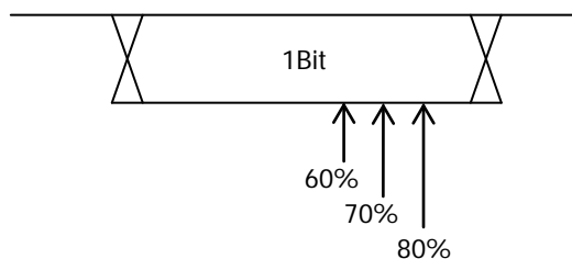
Figure 5-15 Sample Point Position
