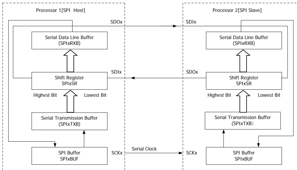
Figure 5-12 SPI Trigger
