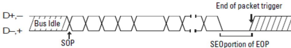
Figure 5-13 USB Trigger
