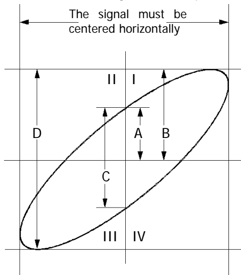
Figure 3-2 Measurement Schematic Diagram of the Phase Deviation
