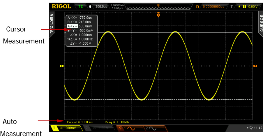
Figure 6-8 Manual Cursor Measurement Example
