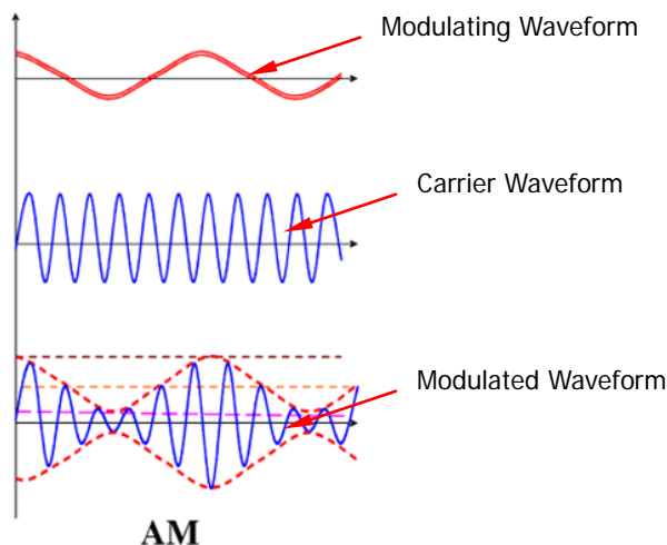
Figure 12-9 AM
