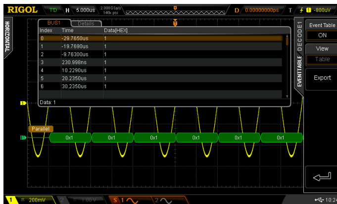
Figure 7-2 Parallel Decoding Table
