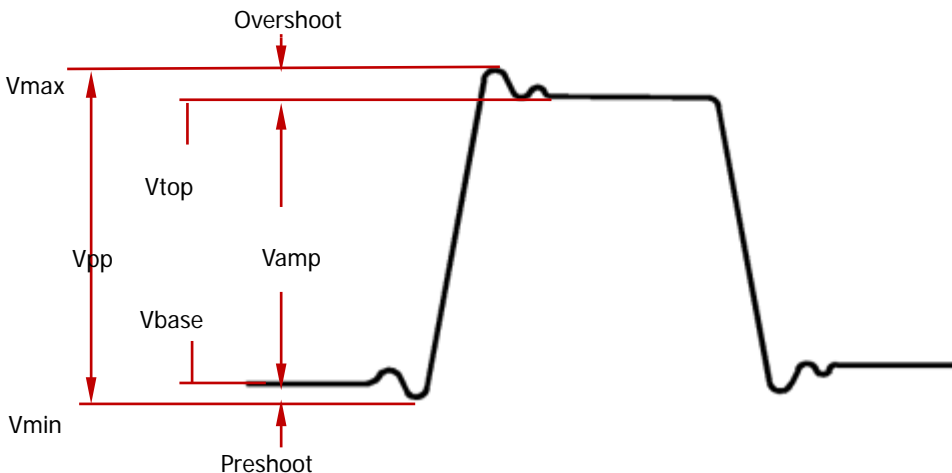
Figure 6-5 Voltage Parameters
