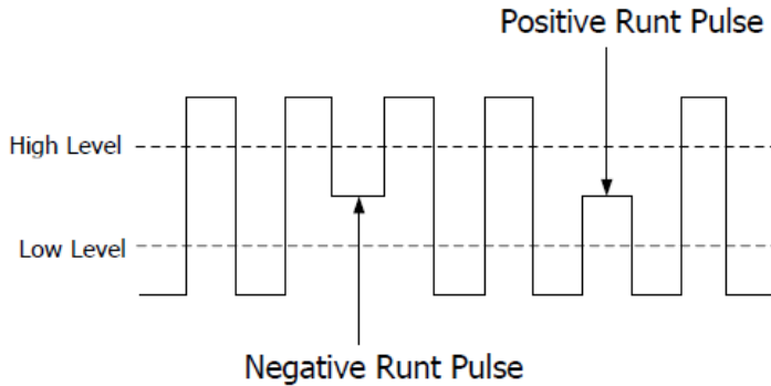
Figure 5-3 Runt Trigger
