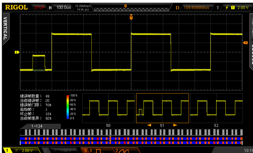
Figure 10-2 Analyze the waveform recorded
