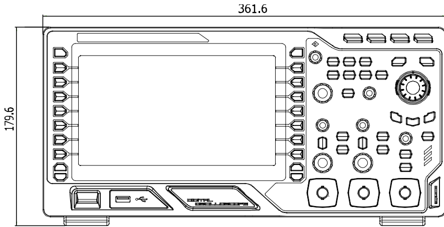
Figure 1-1 Front View
