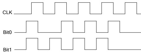
Figure 7-1 Parallel Decoding
