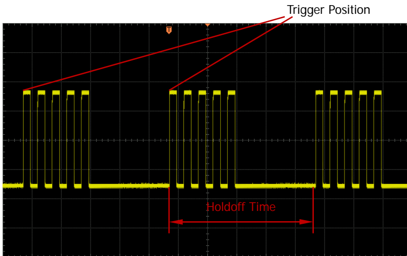
Figure 5-2 Holdoff Time
