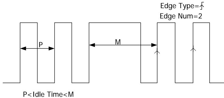
Figure 5-4 Nth Edge Trigger
