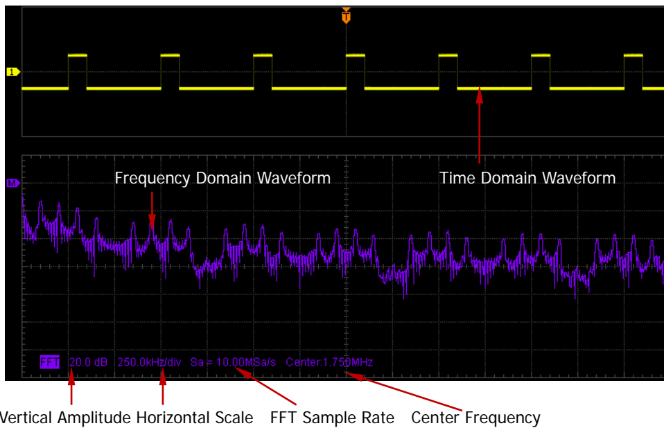
Figure 6-1 FFT
