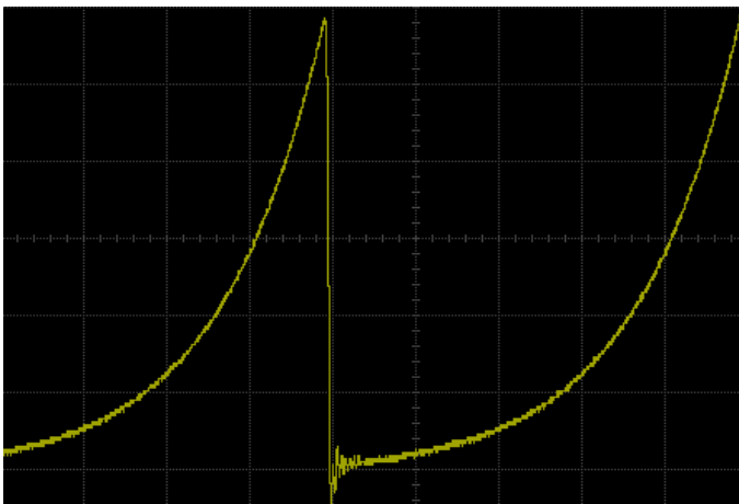
Figure 12-3 ExpRise Function Waveform
