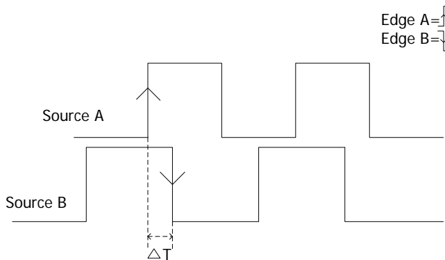
Figure 5-6 Delay Trigger
