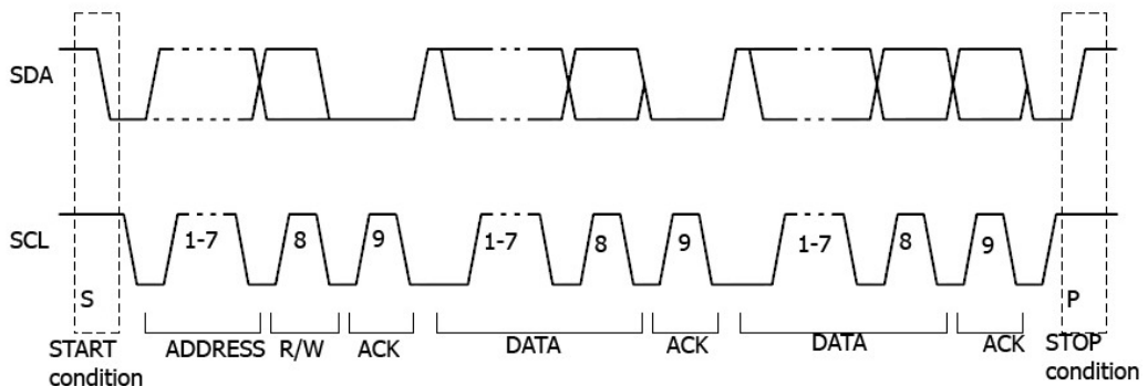
Figure 5-11 I2C Trigger
