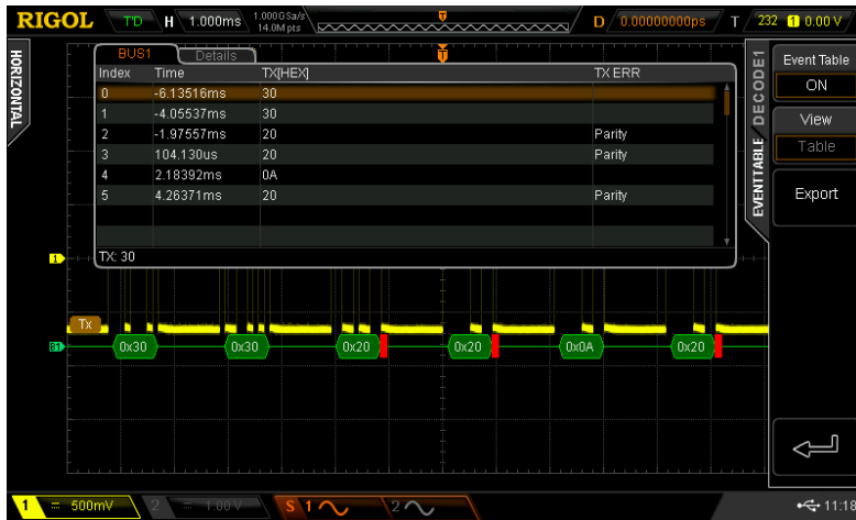
Figure 7-5 RS232 Decoding Table
