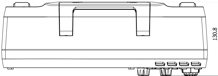
Figure 1-2 Top View
