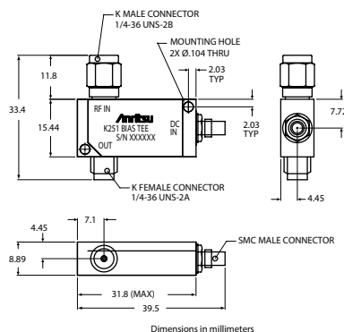
K251 outline
