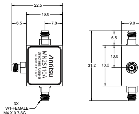
MN25110A outline
