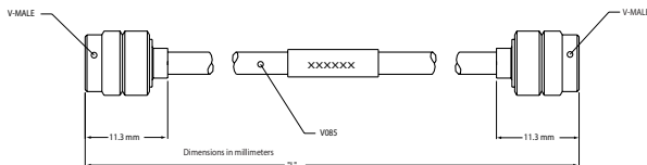
V120MM outline
