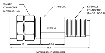
34VKF50 outline
