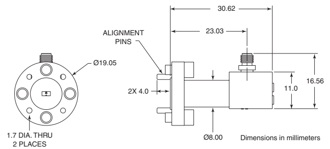
35WR10WF outline
