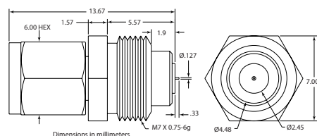
W1-102M, W1-105M ① W1 Male Sparkplug Connector, DC-110 GHz
