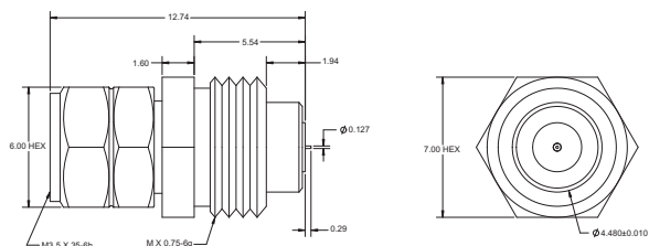
0.8 mm-105M 0.8 mm Male Sparkplug Connector
