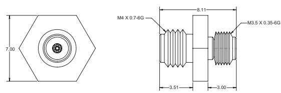
W1 Female to 0.8 mm Female Adapter (33WF.8F50)
