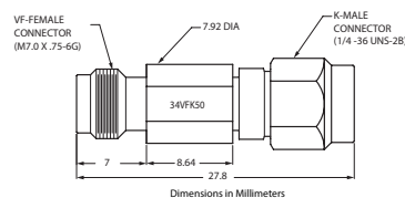
34VFK50 outline
