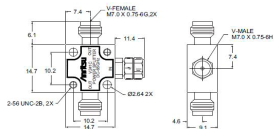
V241C outline
