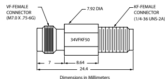
34VFKF50 outline
