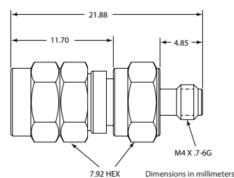
34WVF50 outline
