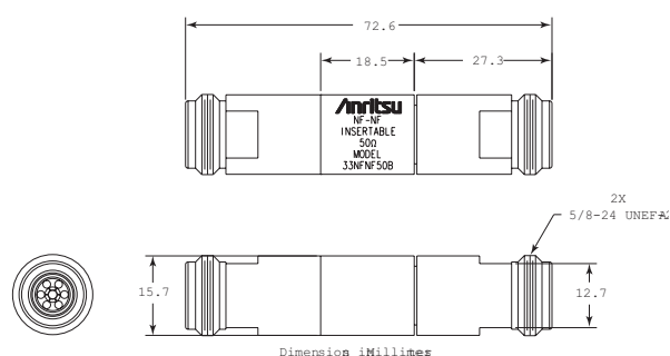
33NFF50B outline
