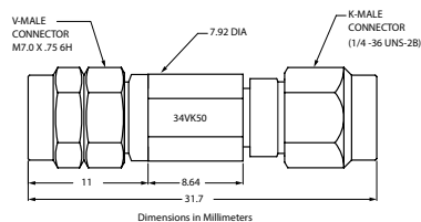
34VK50 outline
